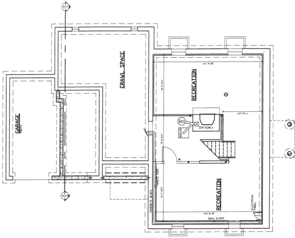
○ BASEMENT/FOUNDATION PLAN
