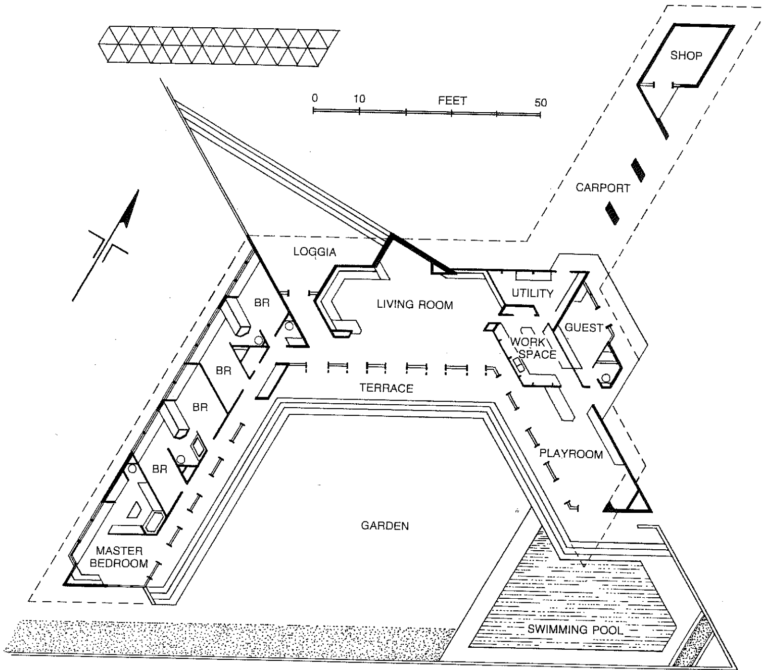
The floorplan of the Fawcett house is a splayed U based on equilateral triangles.
