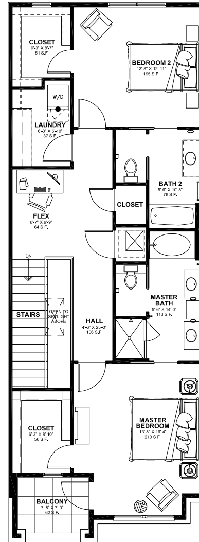
ALDRIDGE - 4D SECOND FLOOR PLAN
