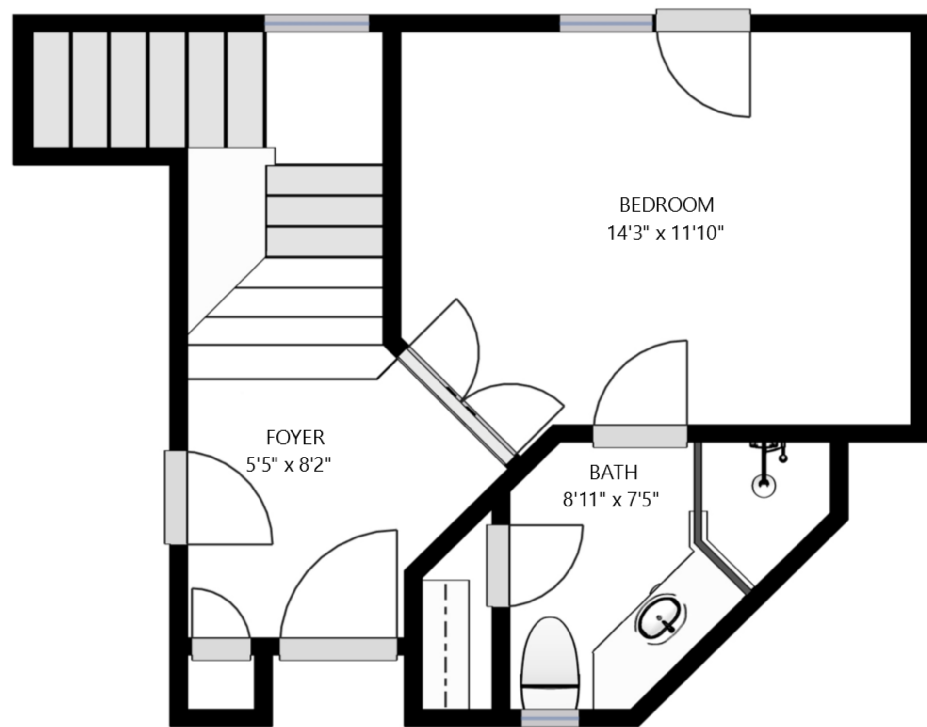
FLOOR 1
