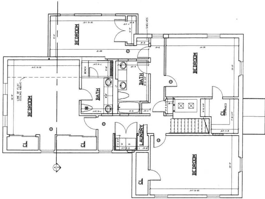
○ SECOND FLOOR PLAN SCALE: 1/4" = 1'-0"
