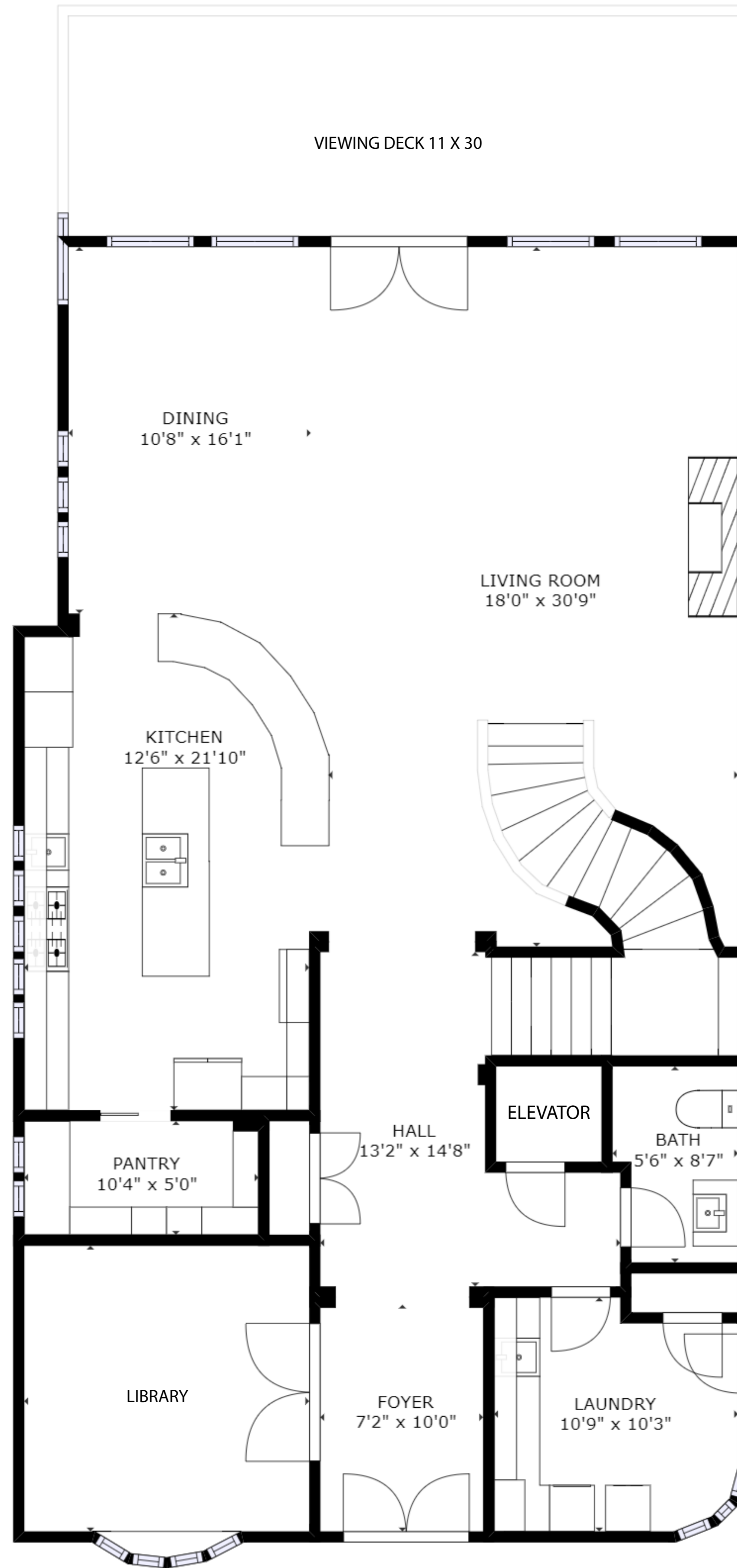
FLOOR 2
