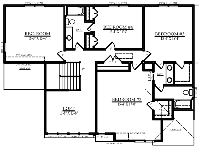
SECOND FLOOR PLAN SCALE: 1/4"=1'-0" 9'-0" CLG. HGT. U.N.O. SET WINDOWS @ 7'-10" U.N.O. 1551 SQ. FT.
