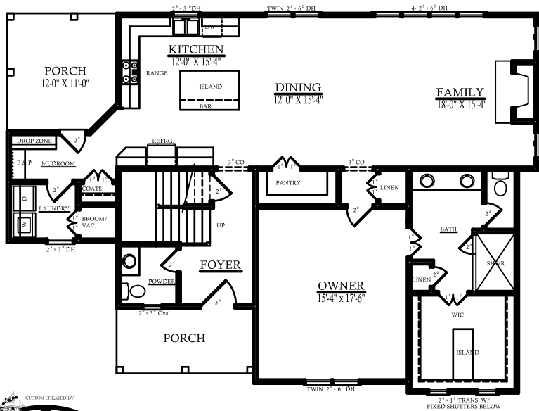
FIRST FLOOR PLAN SCALE: 1/4"=1'-0" 9'-0" CLG. HGT. U.N.O. SET WINDOWS @ 7'-10" U.N.O. 1611 SQ. FT. PRELIMINARY DESIGN SUBJECT TO CHANGE
